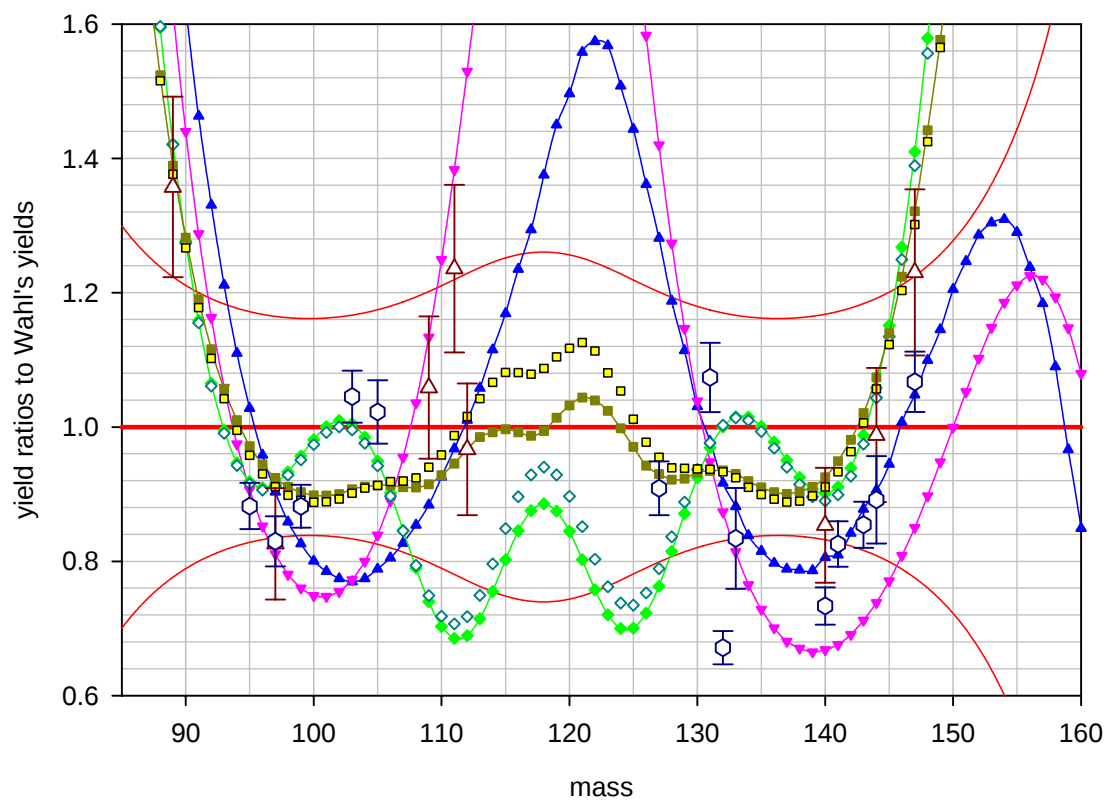
Benchmark A: ^{239}\text{Pu} at 14-15 MeV, post neutron emission yield ratios to Wahl's systematics Further partial plots to show more details; lower graph: for legend see upper graph
